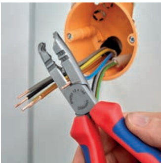
Cutting when shortening single conductors
