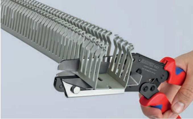
Blade length 110 mm for cutting wide cable ducts
